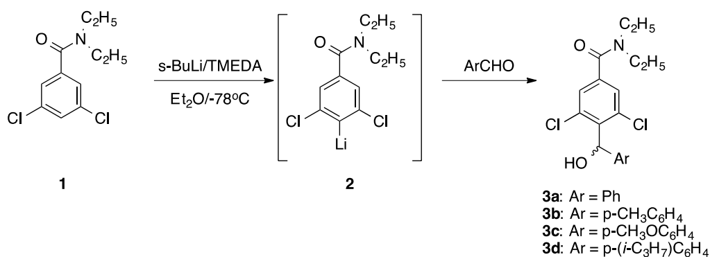
Scheme 1. Para -Metalation/elaboration of a tertiary 3,5-dichlorobenzamide.
