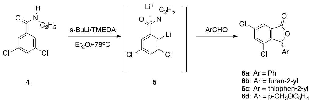
Scheme 2. Ortho-Metalation/elaboration of a secondary 3,5-dichlorobenzamide.
